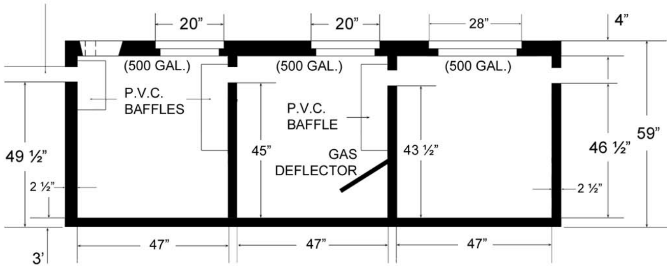
SIDE VIEW
