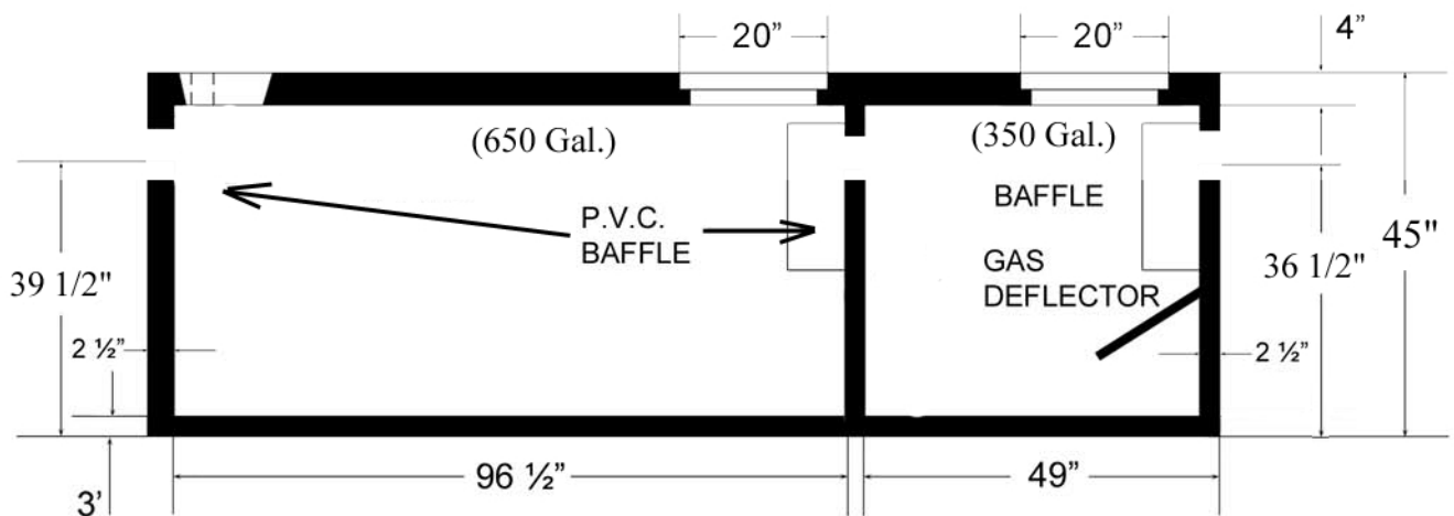
SIDE VIEW
