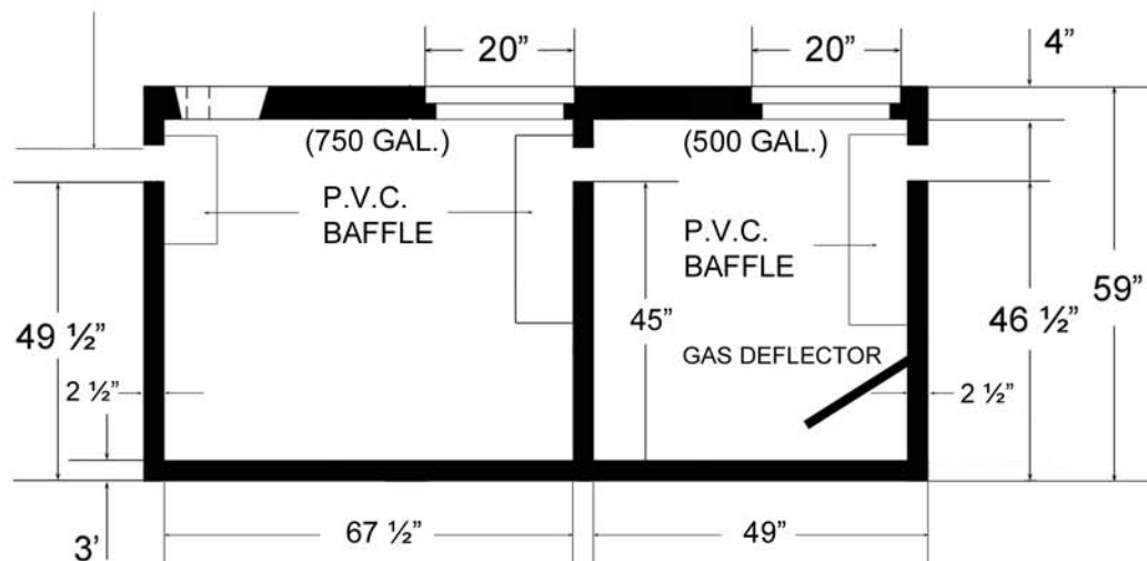
SIDE VIEW
