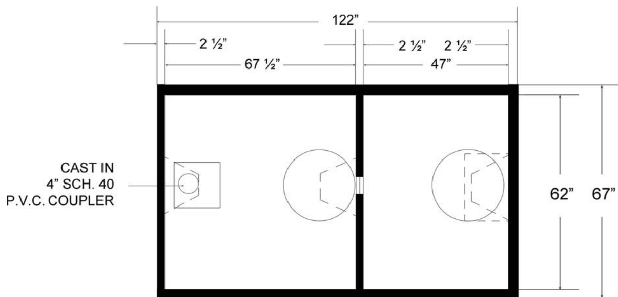
TOP VIEW
