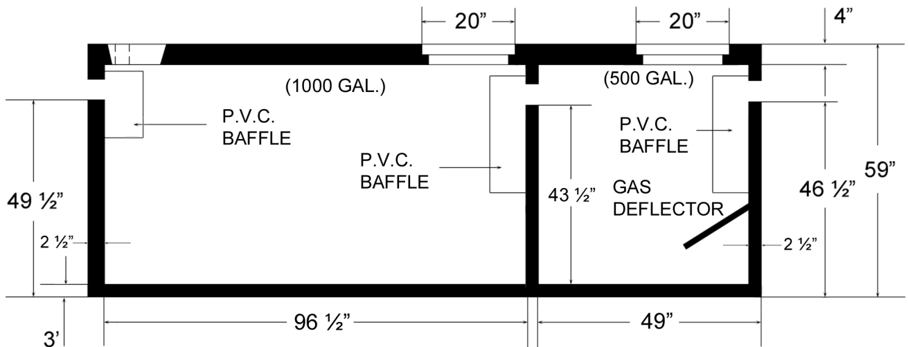
SIDE VIEW
